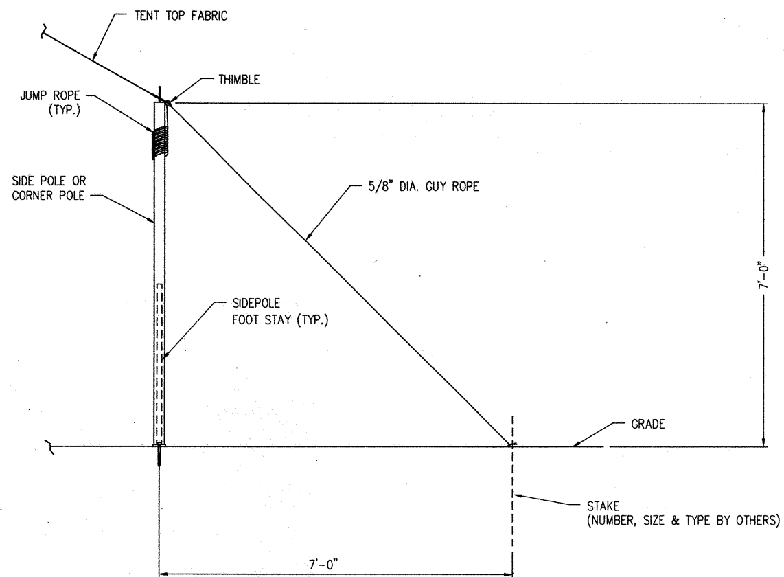
DETAIL AT INTERMEDIATE GUYS
