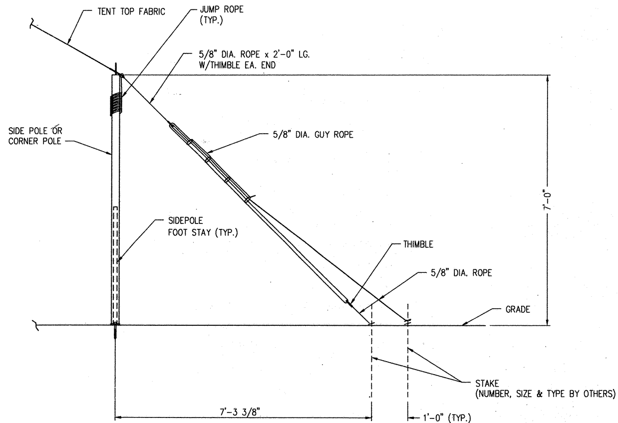
DETAIL AT CORNERS, LACE LINES, & CENTER ENDS
