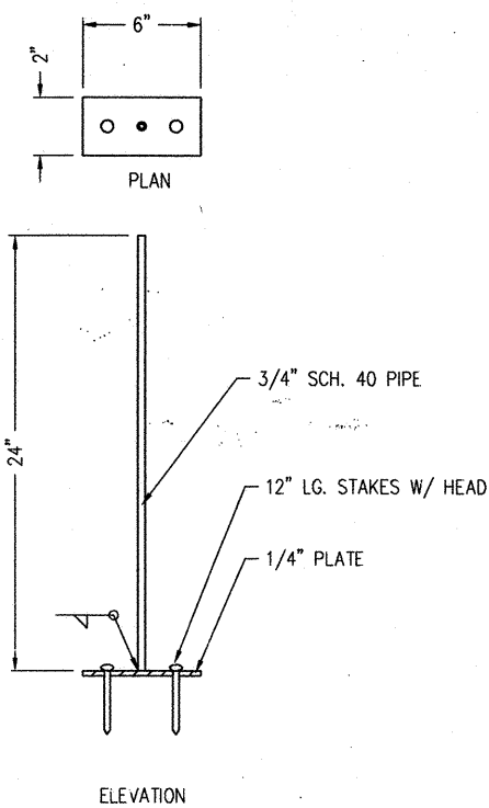
SIDE POLE FOOT STAY DETAIL
