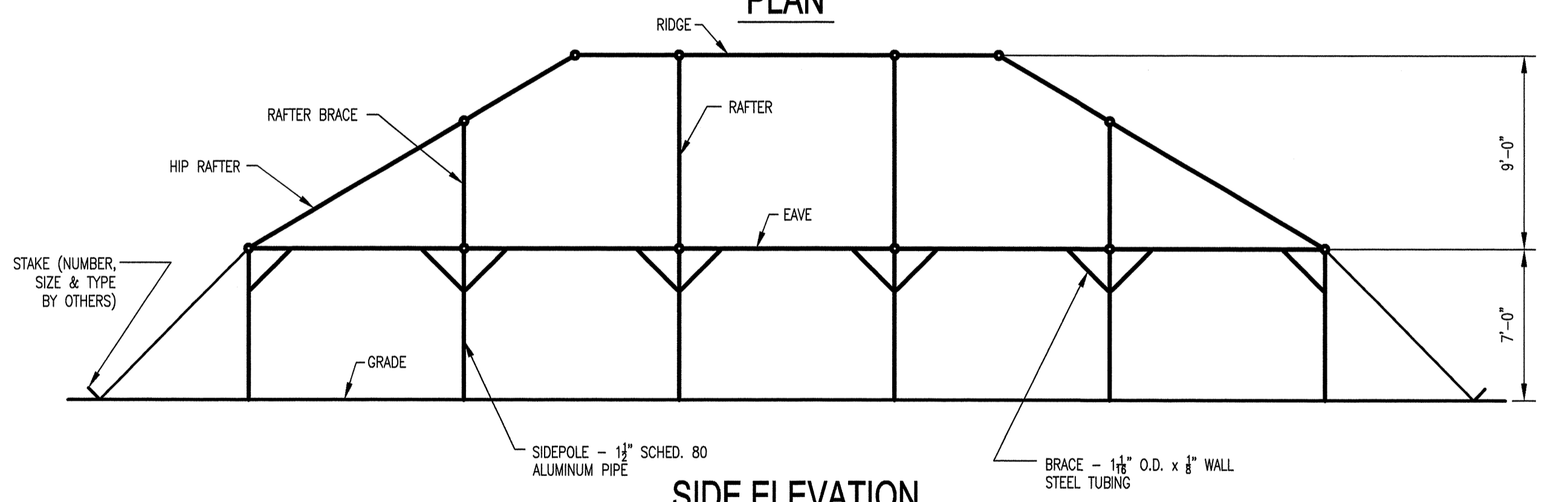
SIDE ELEVATION
