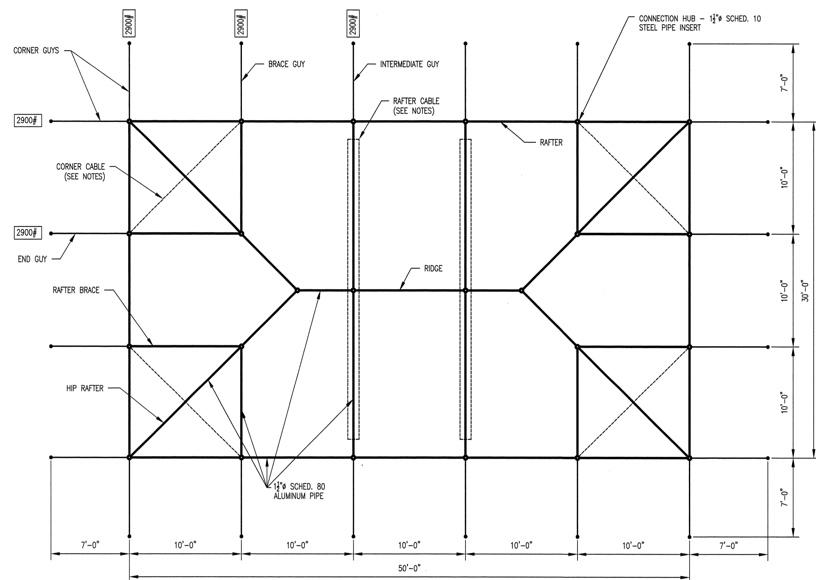
PLAN
