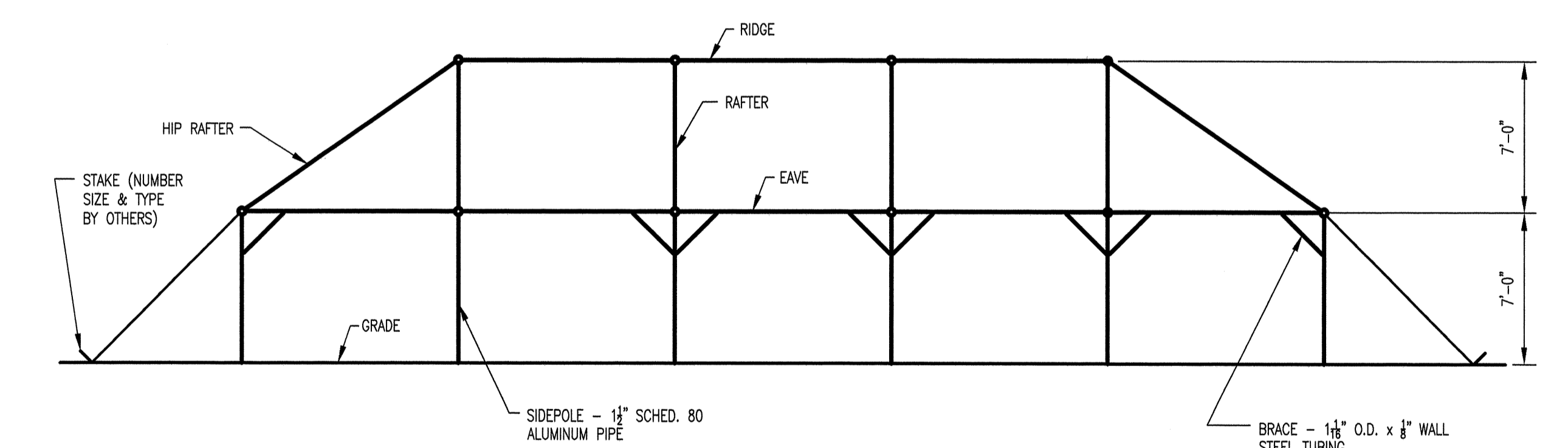
SIDE ELEVATION
